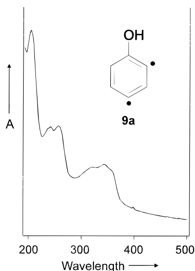
Figure 4. UV-vis spectrum of didehydrophenol 9a in argon at 10 K.
